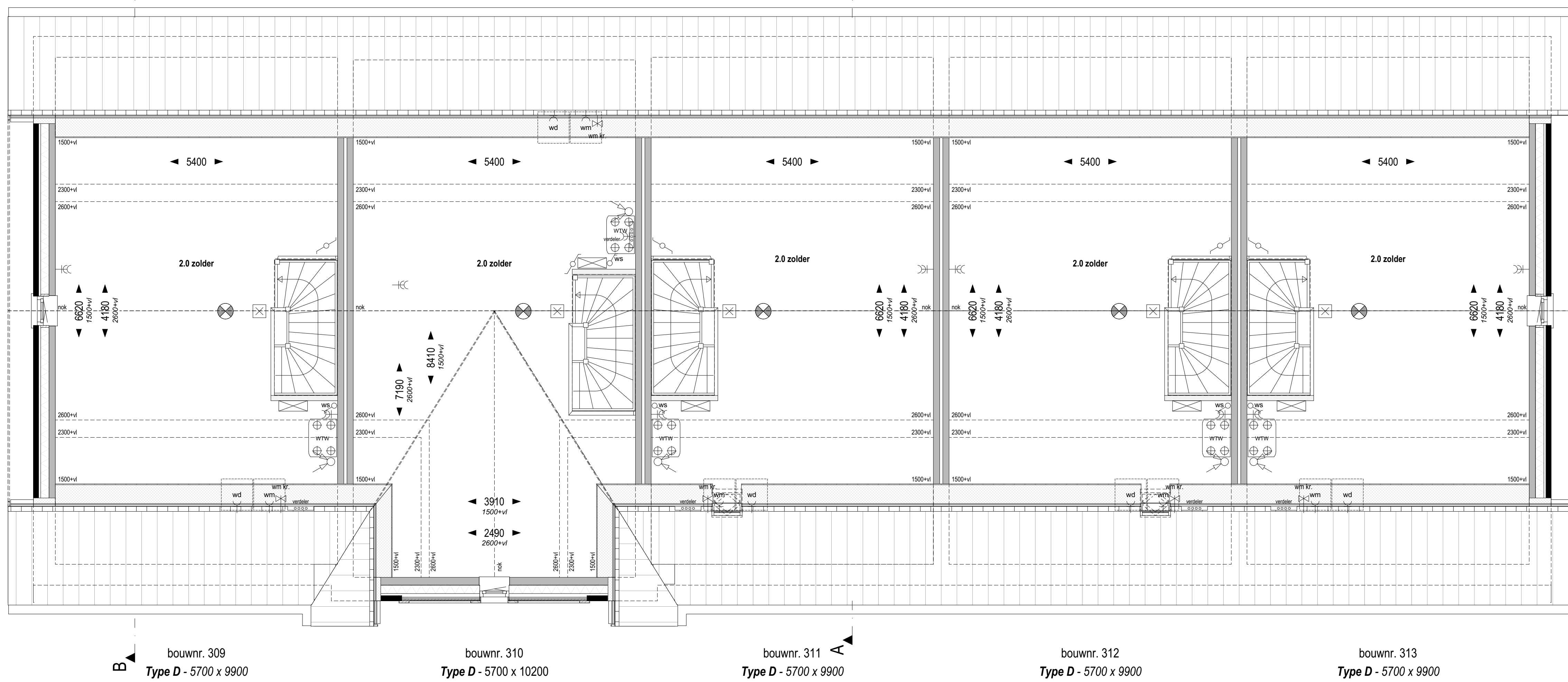
Zolder +5.840 (1:50)
