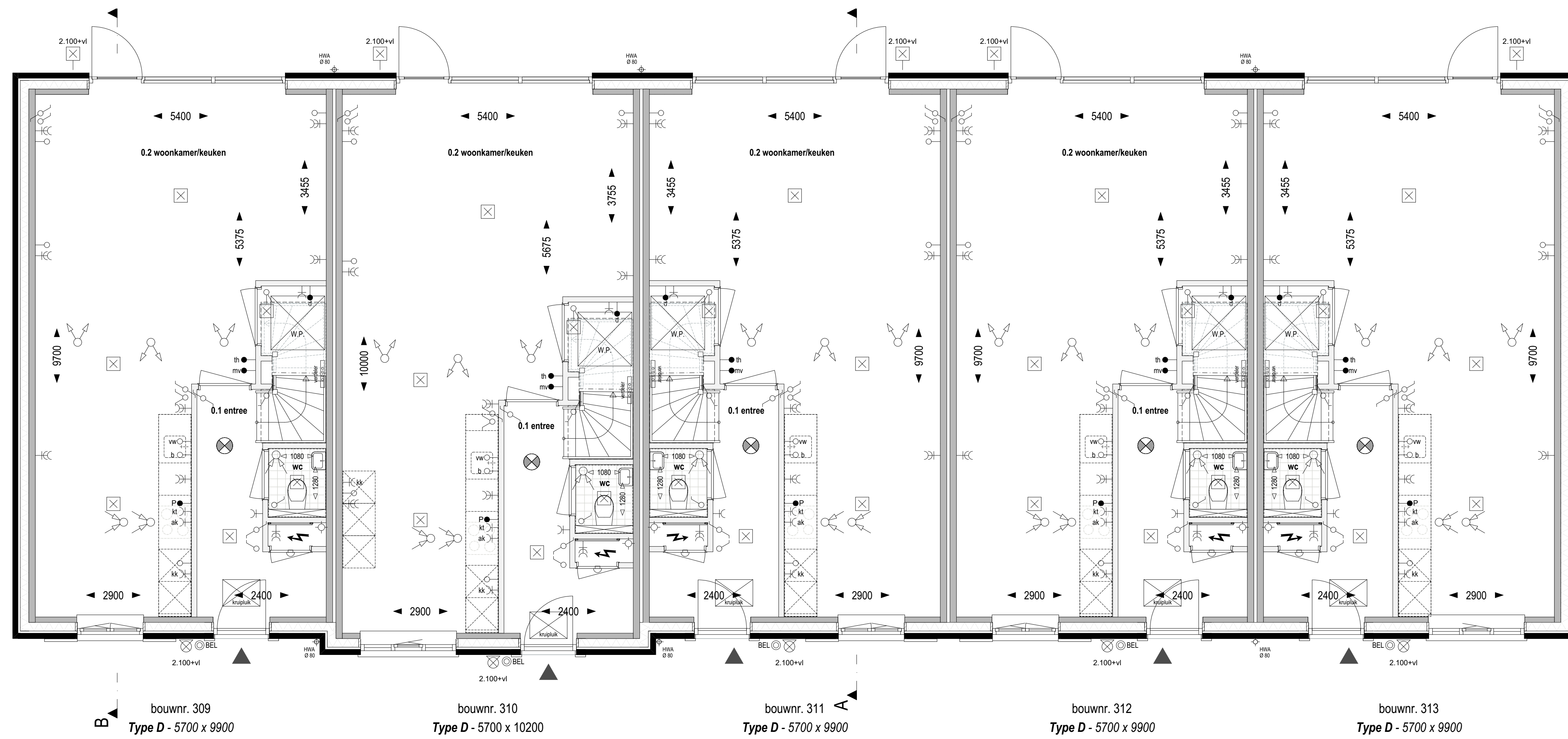
Begane grond Peil=0, (1:50)
